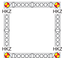
MAXIMUM four manual chain hoists
