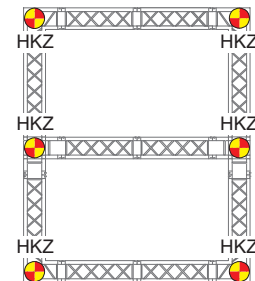
MAXIMUM four manual chain hoists
