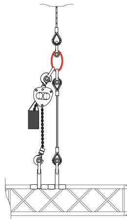
END HEIGHT manual chain hoist
